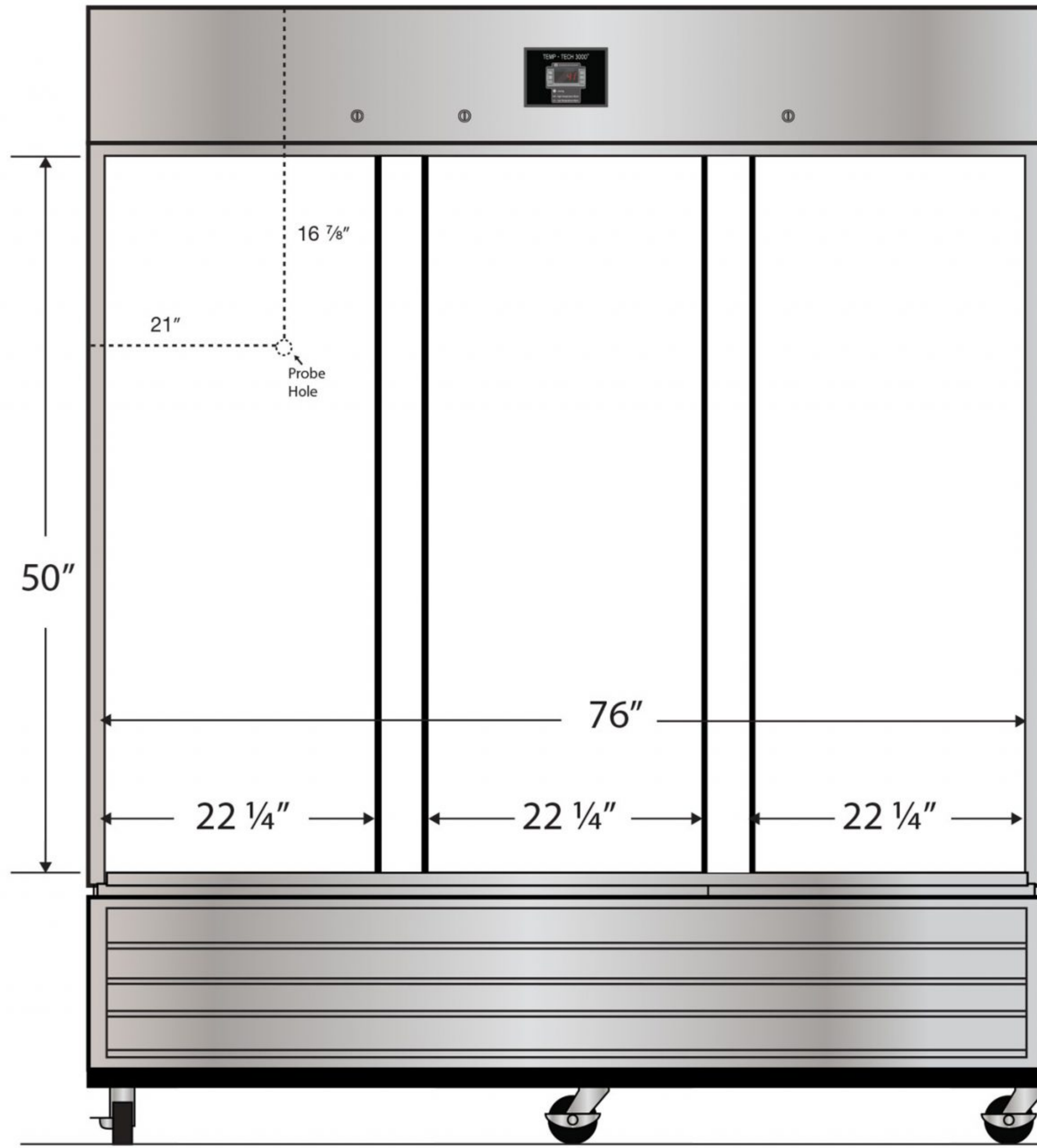
Front View
