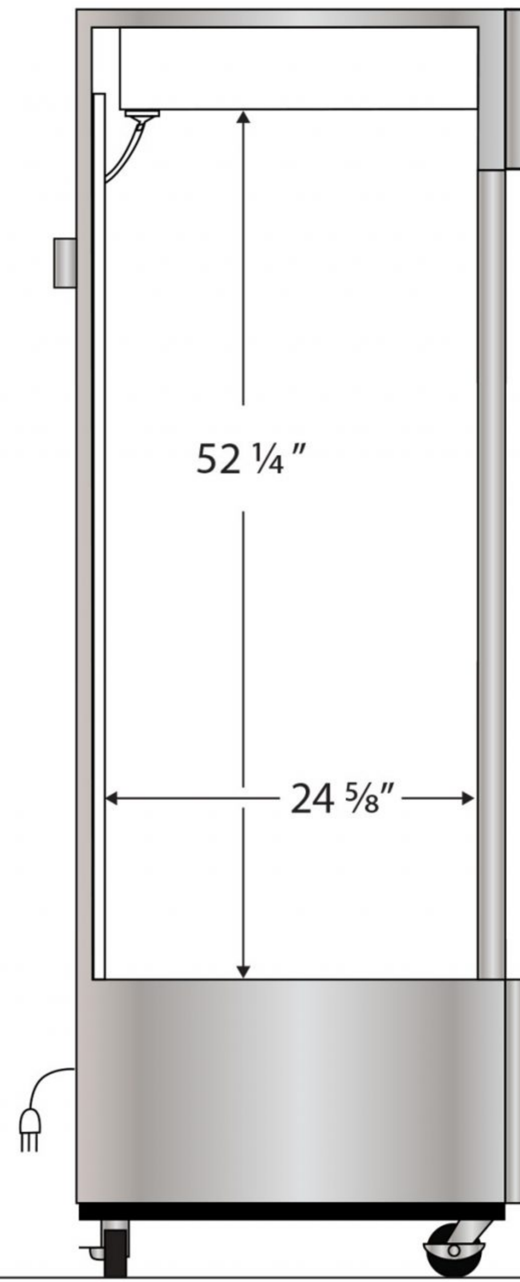
Side View
