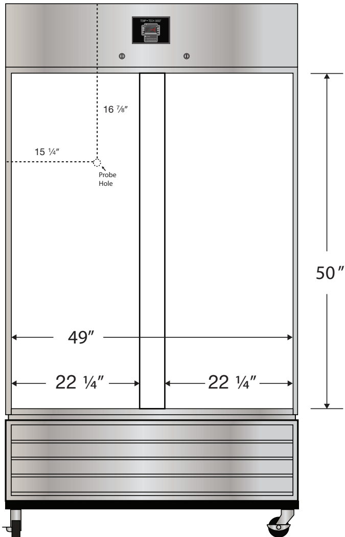
Front View
