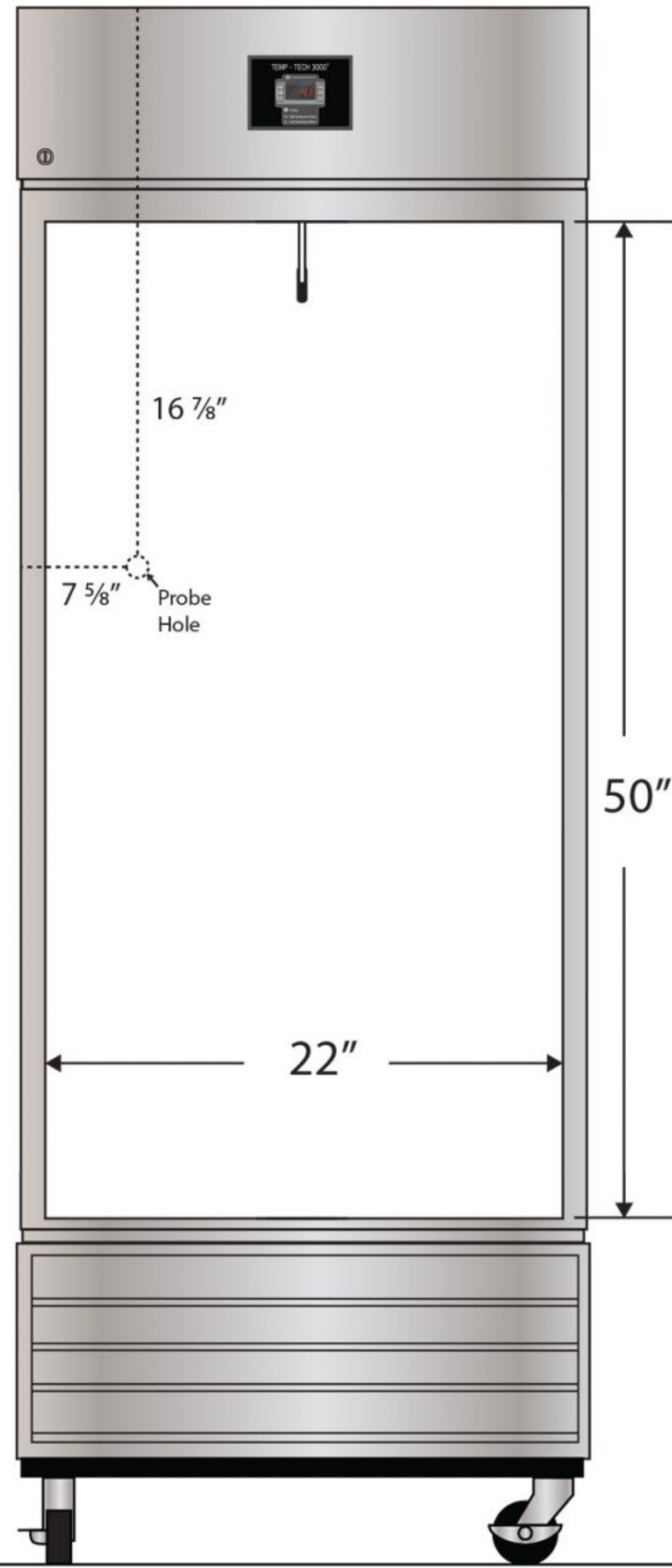
Front View
