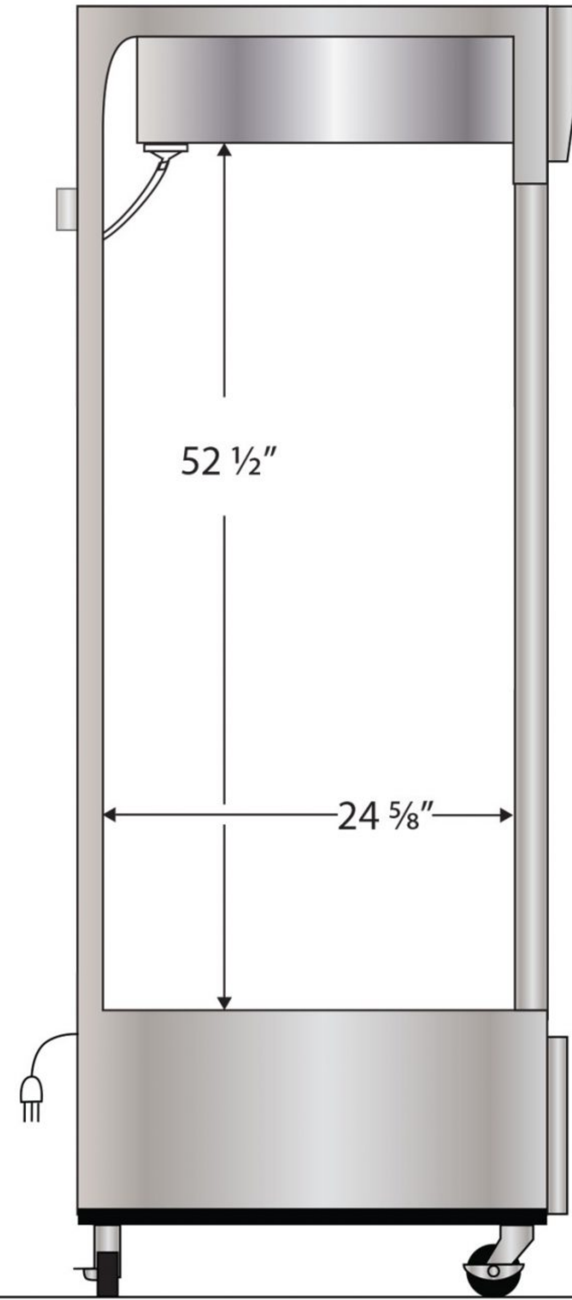
Side View
