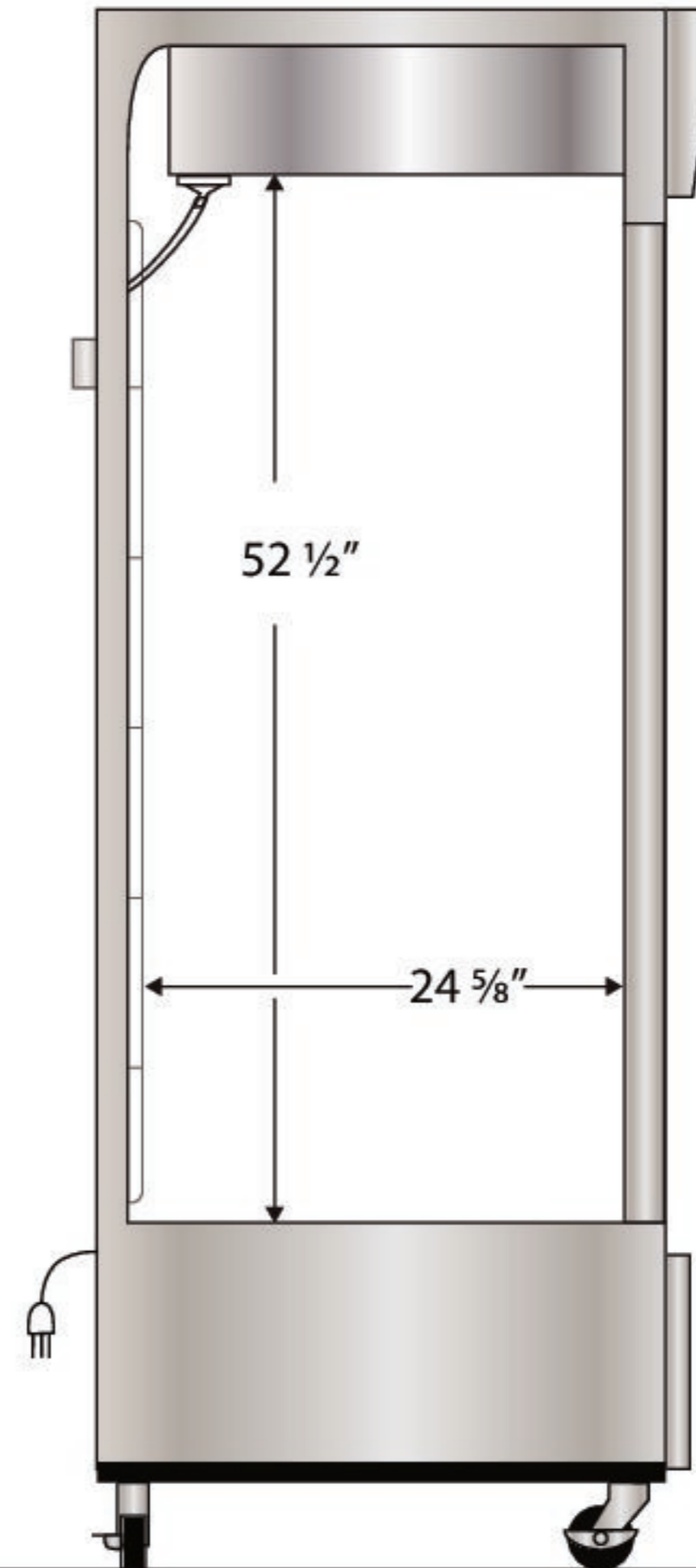
Side View
