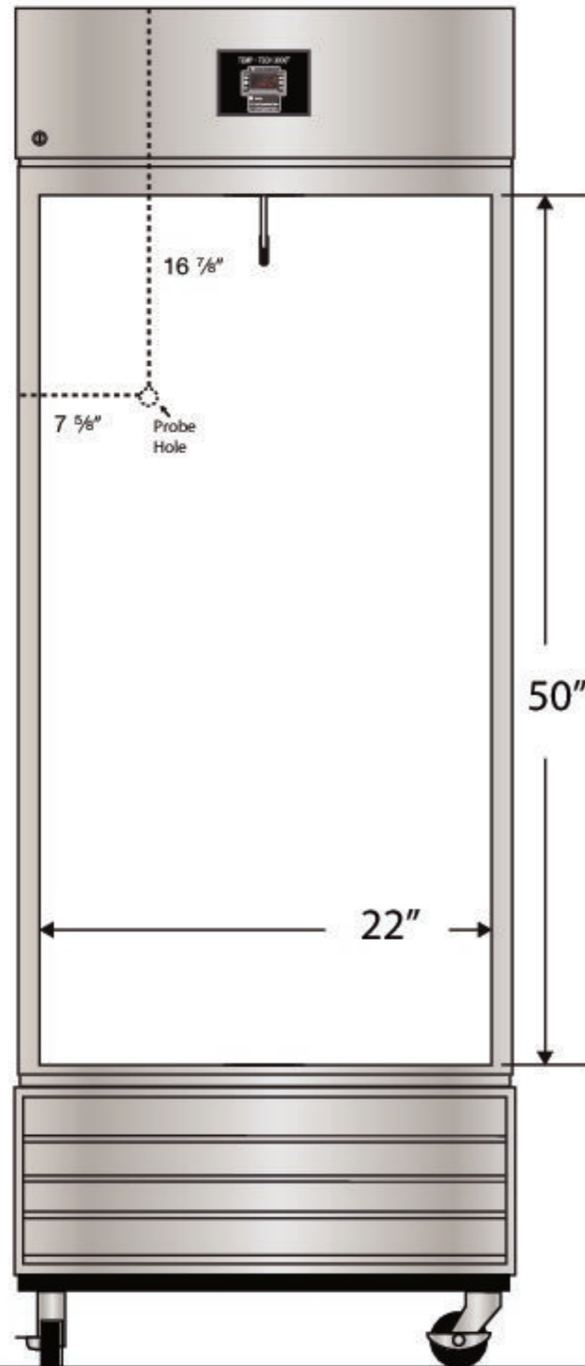
Front View
