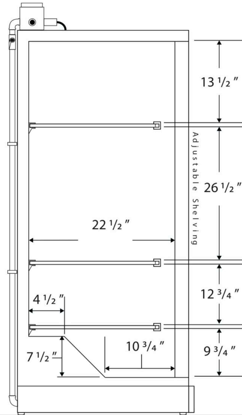
Side View
