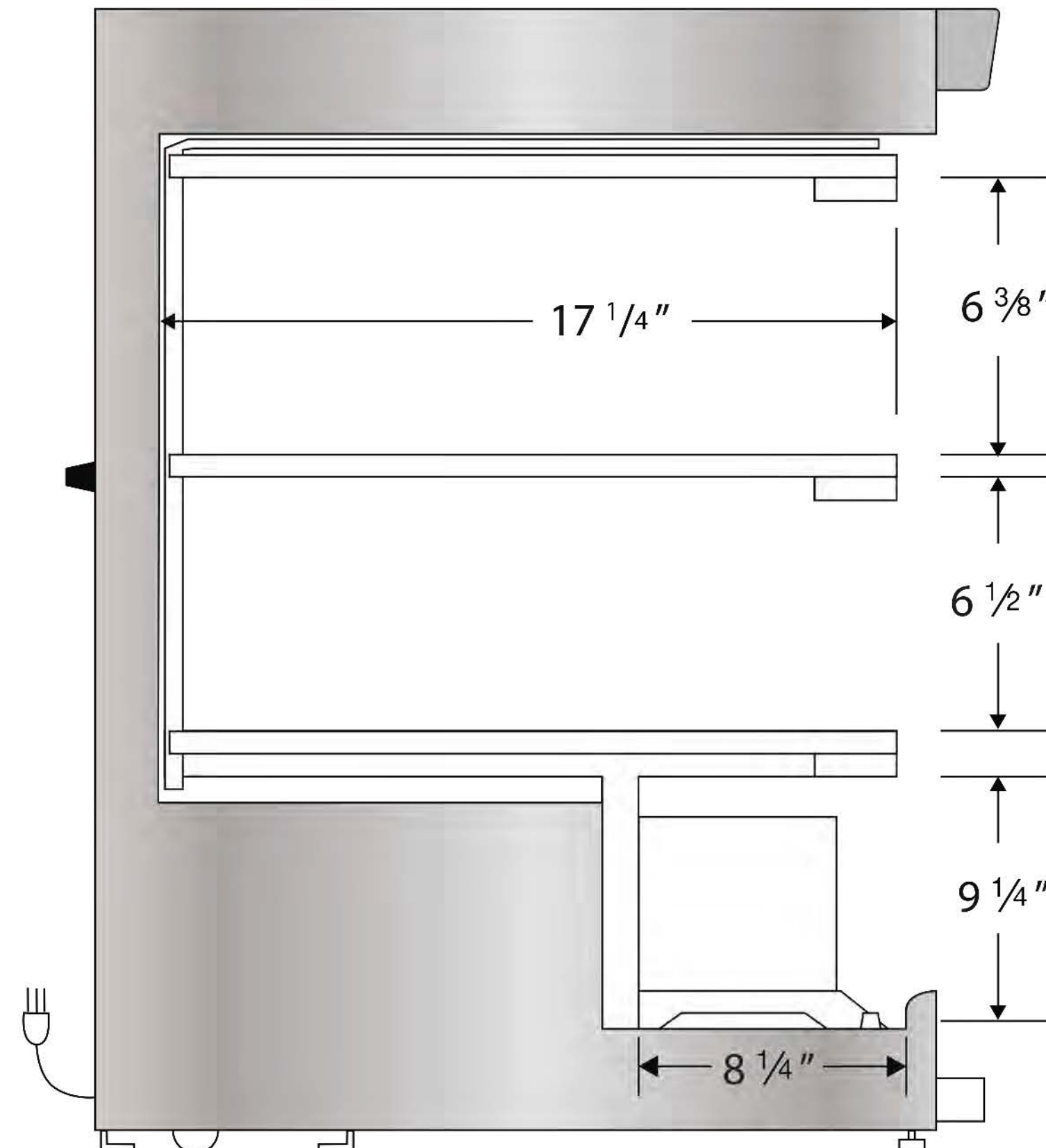
Side View
